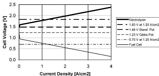
Fig. 2. Voltage-current characteristics of hydrogen electrolyzer and fuel cell.
